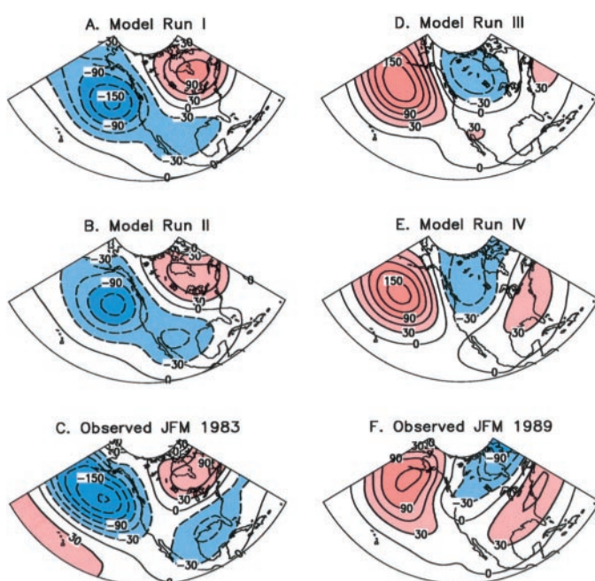
Fig. 3. Average 500-millibar (0.05 MPa) height anomaly (meters) for JFM for integrations with observed SST in 1982–1983 starting from atmospheric initial conditions in mid-December 1982 (A) and 1988 (B) and observed (C), and with observed SST in 1988–1989 from initial conditions in mid-December 1982 (D) and 1988 (E) and observed (F).
